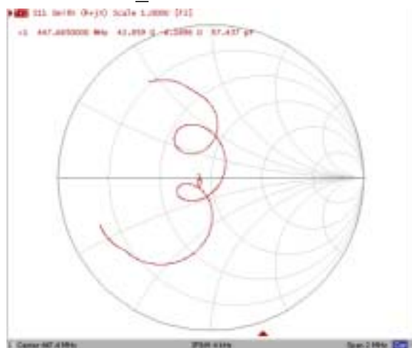
Smith Chart_S11 :
